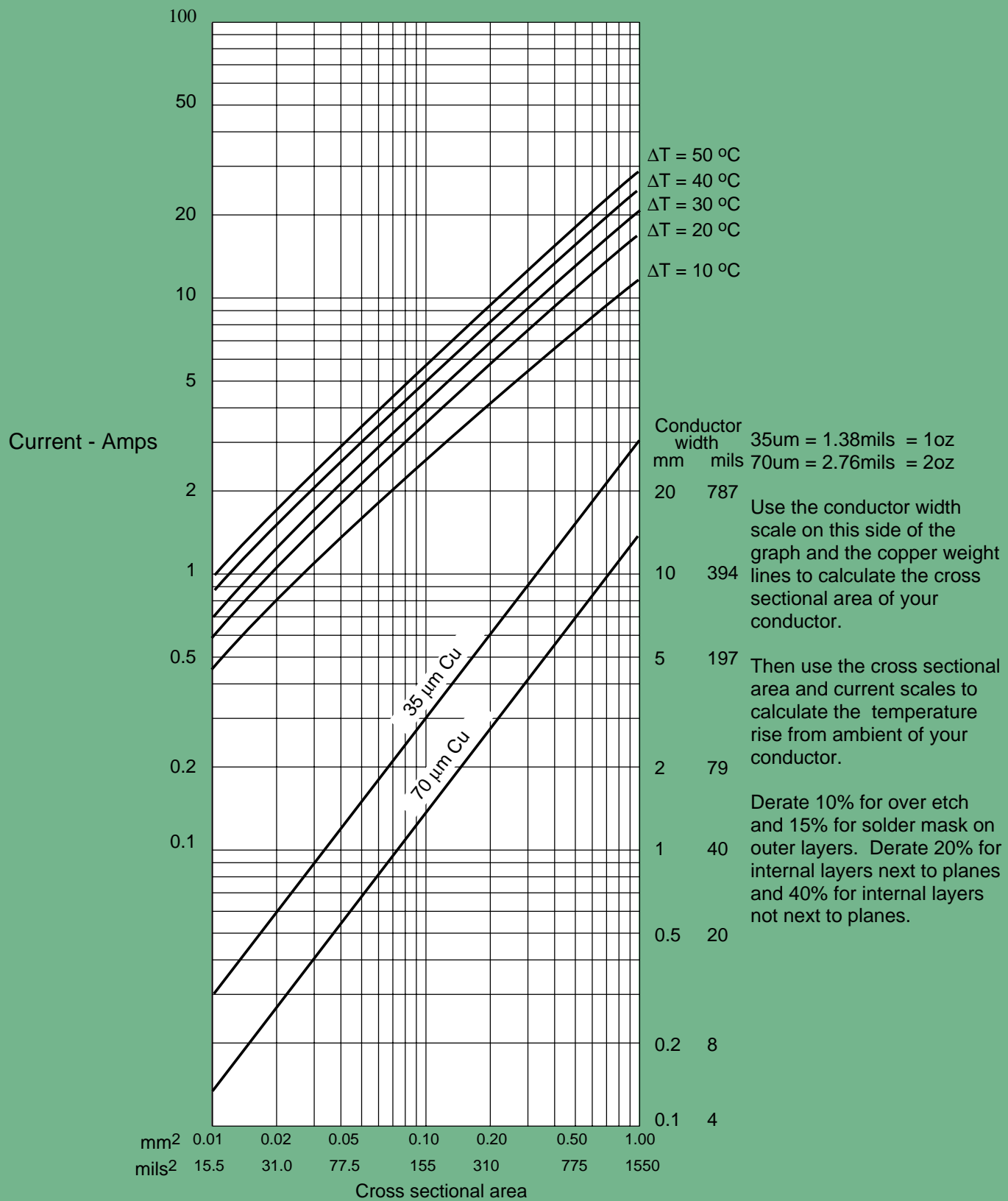
Relation between current, dimensions of tracks in PCBs and temperature rise.
