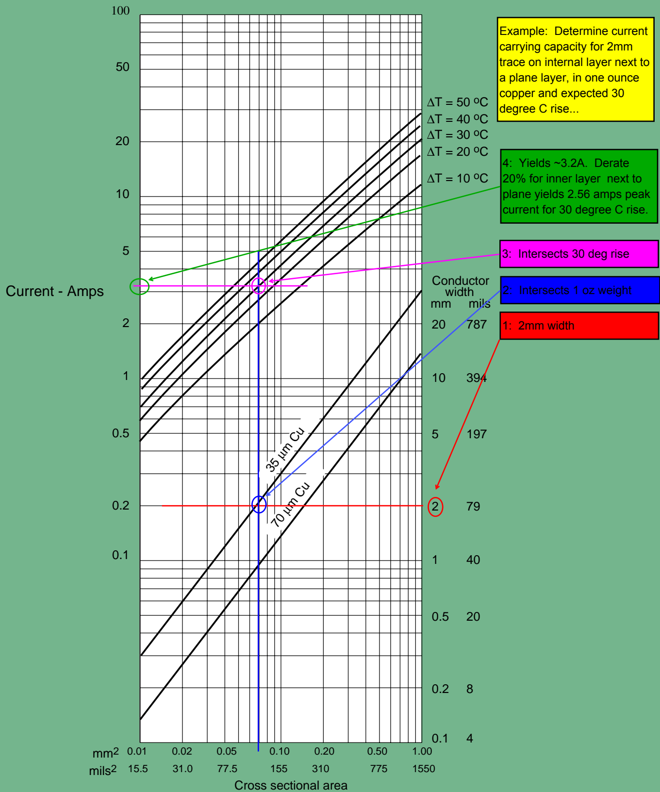
Relation between current, dimensions of tracks in PCBs and temperature rise.
