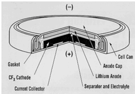
Figure 3. Construction of a Lithium Carbon Monofluoride Coin Cell.
