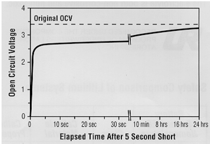
Figure 8. Short Circuit Recovery of a Lithium Carbon Monofluoride Coin Cell.
