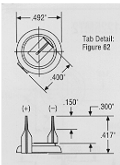
Figure 7. Tabbed BR1225 Lithium Coin Cell.
