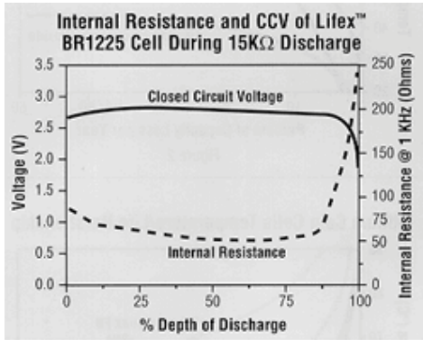
Figure 2. Closed Circuit Voltage and Internal Resistance Over Discharge.
