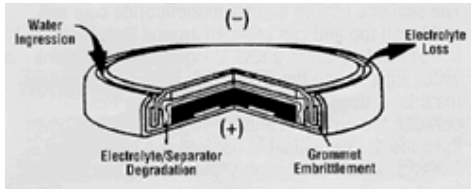
Figure 1. High Temperature Failure Modes of Lithium Coin Cells.
