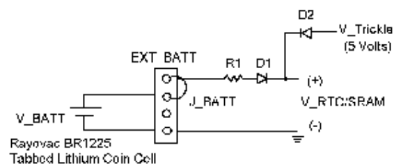
Figure 9. RTC/SRAM Circuit Using a Rayovac BR1225 and a Trickle/Standby Power Supply.
