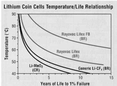
Figure 4. Effects of Thermal Wear Out on Lithium Coin Cells.
