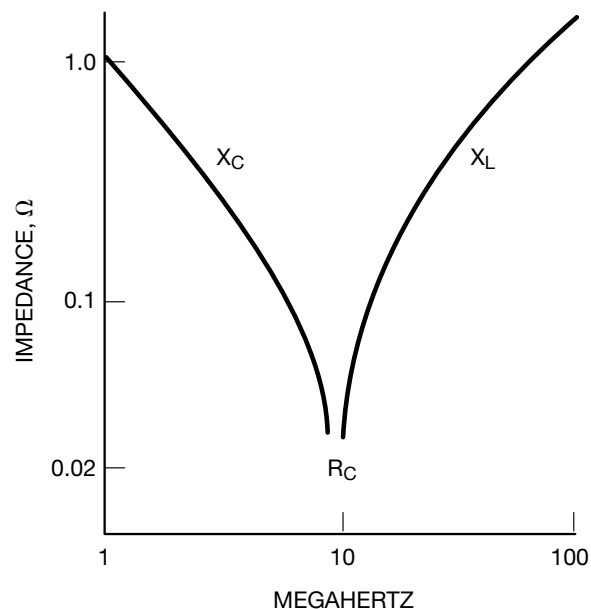
Fig. 6. Major impedance components
