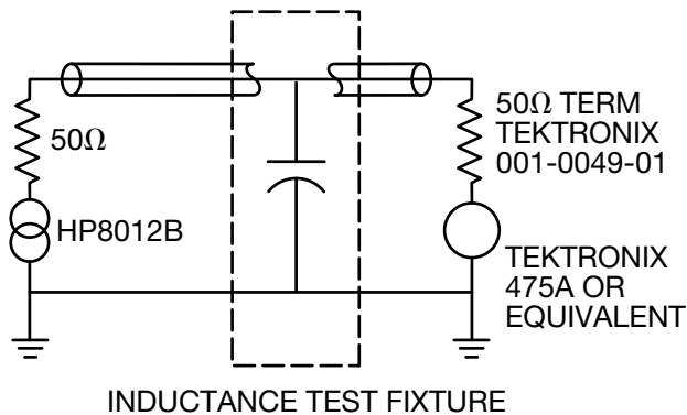
Fig. 7. High-frequency test schematic
