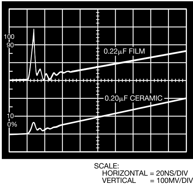
Fig. 12. Comparison of 0.2- \mu F MLC with 0.22- \mu F film capacitor
