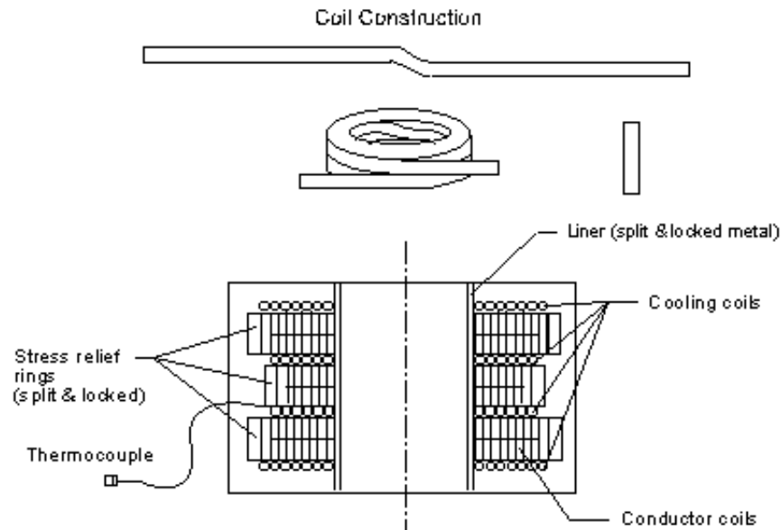
Figure 4. "Supercoil" Fixture
