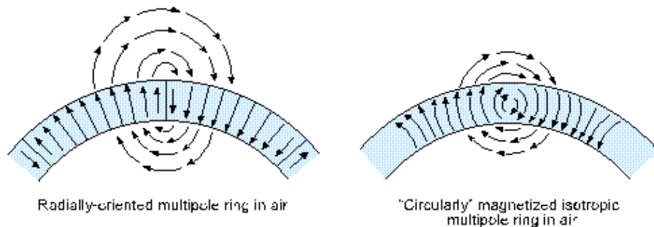
Figure 7. "Circular" Pole Transitions
