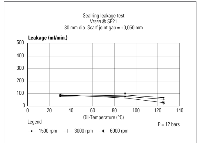
Fig. 50 SP21 Seal ring. Scarf joint gap
