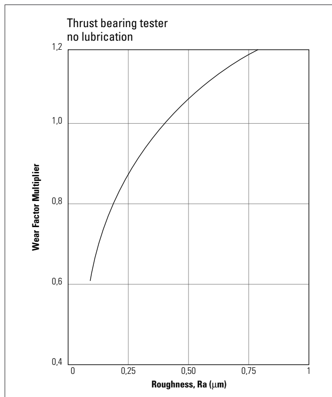
Fig. 42 Effect of mating material surface finish on wear
