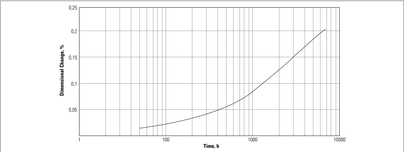
Fig. 23 SP1 and SP21 polyimide shapes. Typical dimensional change vs. time at 23°C, 50% RH, 3,2 mm plaques
