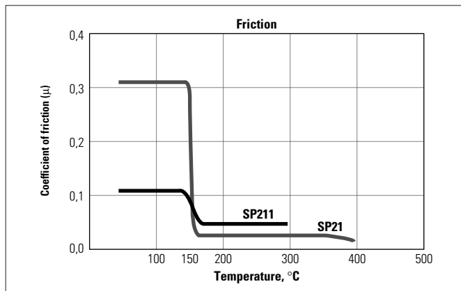
Fig. 39 Coefficient of friction of SP21 and SP211 for unlubricated operation against mild carbon steel
