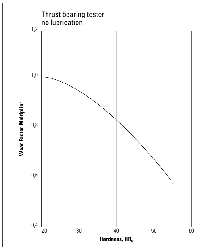
Fig. 41 Effect of mating material hardness on wear
