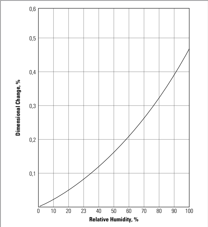
Fig. 26 SP1 anf SP21 polyimide shapes. Typical dimensional change with relative humidity at equilibrium, 23°C
