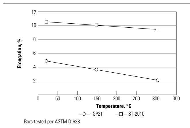
Fig. 7 Ultimate elongation vs. temperature SP21 vs. ST2010
