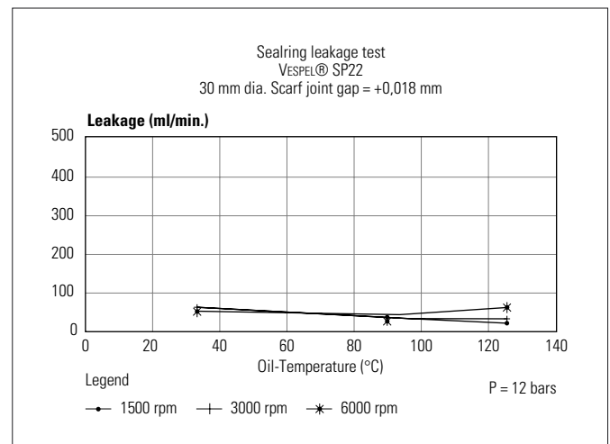
Fig. 51 SP22 Seal ring. Scarf joint gap
