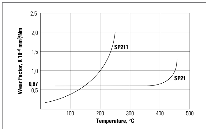
Fig. 40 Wear factor of SP21 and SP211 for unlubricated operation against mild carbon steel
