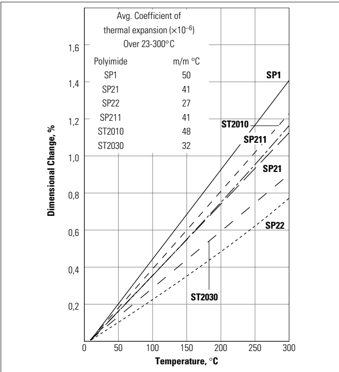
Fig. 29 Direct-formed SP and ST polyimide. Linear expansion (⊥ to forming) ASTM D696
